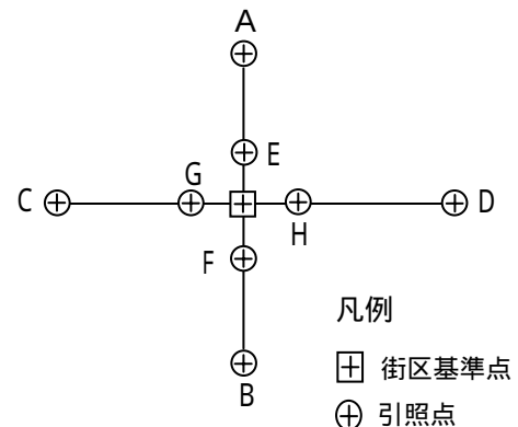
図2-1-2 X型 (E,F,G,Hは補助引照点)
